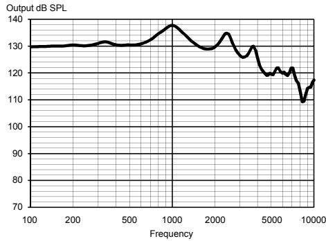
MAXIMUM OUTPUT - EAR SIMULATOR IEC 60118-0
